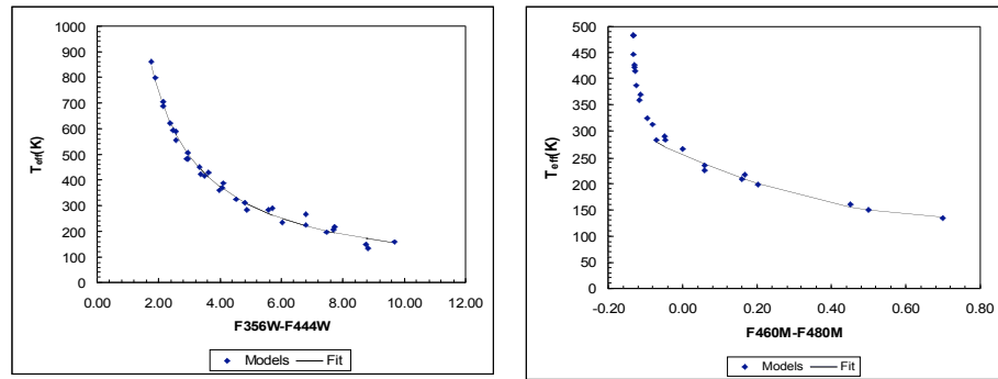
Figure 5: NIRCam will be able to measure the effective temperatures of Jupiter-like planets very well as the plots below illustrate. The “data points” show the result of convolving Burrows et al. models with NIRCam filters to compute the two colors plotted. The color versus temperature relations were fit with simple polynomials and show that these two colors will provide temperature measurements.
