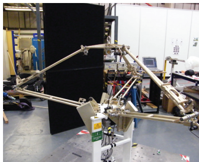
Deployable mast (breadboard) Airbus Defence and Space Limited
