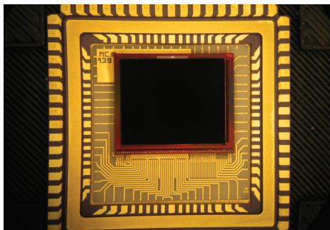
Near-infrared detector (breadboard) ESA/CEA-LETI (Fr)
