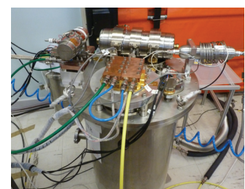
15K pulse tube cooler (breadboard) Air Liquide Advanced Technologies
