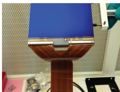
CCD 270 developed by e2v for PLATO ESA
