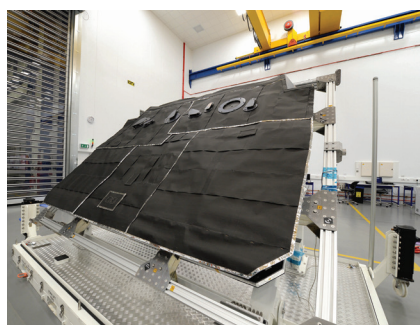
Structural and thermal model of heat shield for Solar Orbiter Airbus Defence and Space 2015
