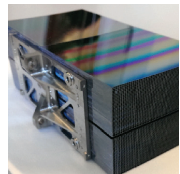
Silicon Pore Optics mirror module ESA/cosine Research
